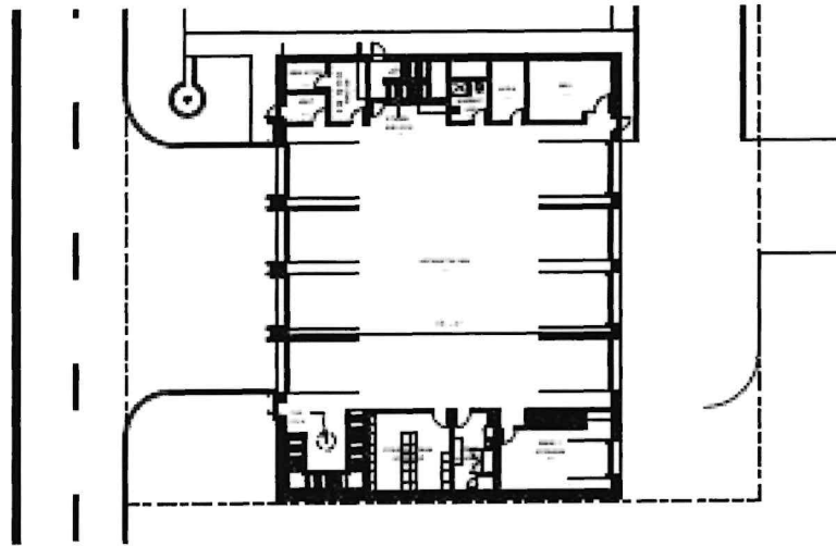
MUNCIE FIRE DEPARTMENT - STATION 5 FIRST FLOOR PLAN RD/11/121 RQAW
